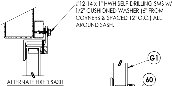
ALTERNATE FIXED SASH
