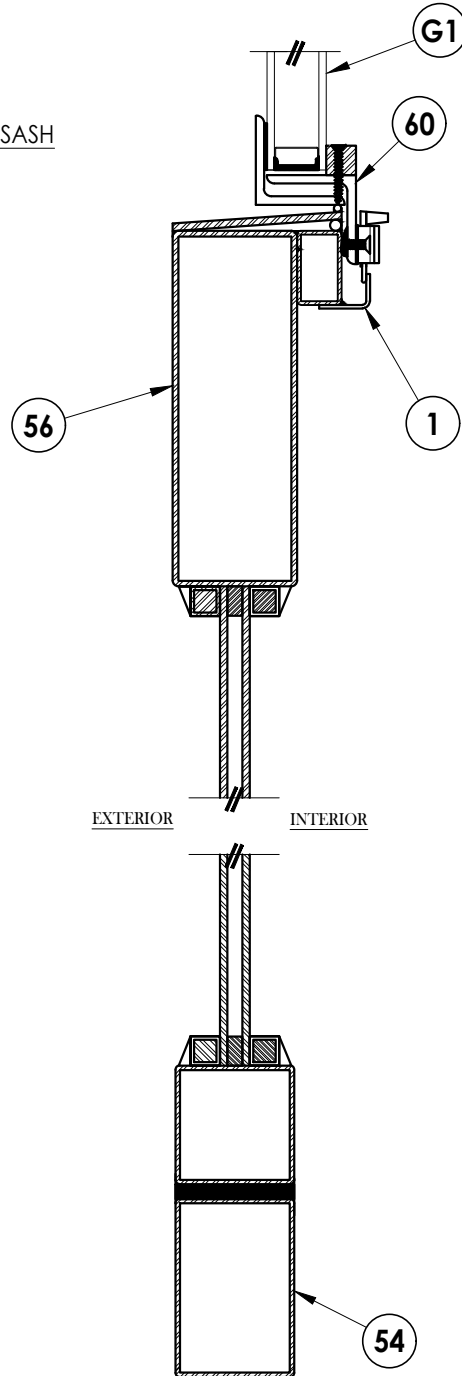
4 VERTICAL CROSS SECTION
