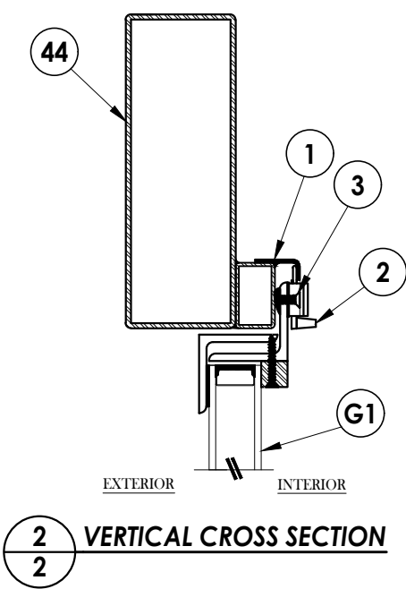
ALTERNATE FIXED SASH
