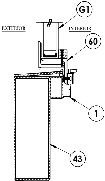
3/2 VERTICAL CROSS SECTION
